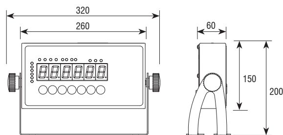
Dimensions (mm)
