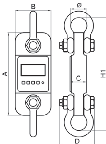
Dimensions (mm)
