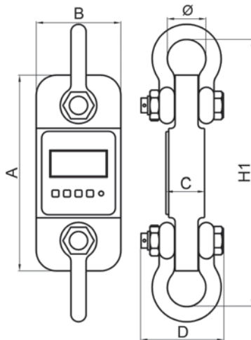
Dimensions (mm)
