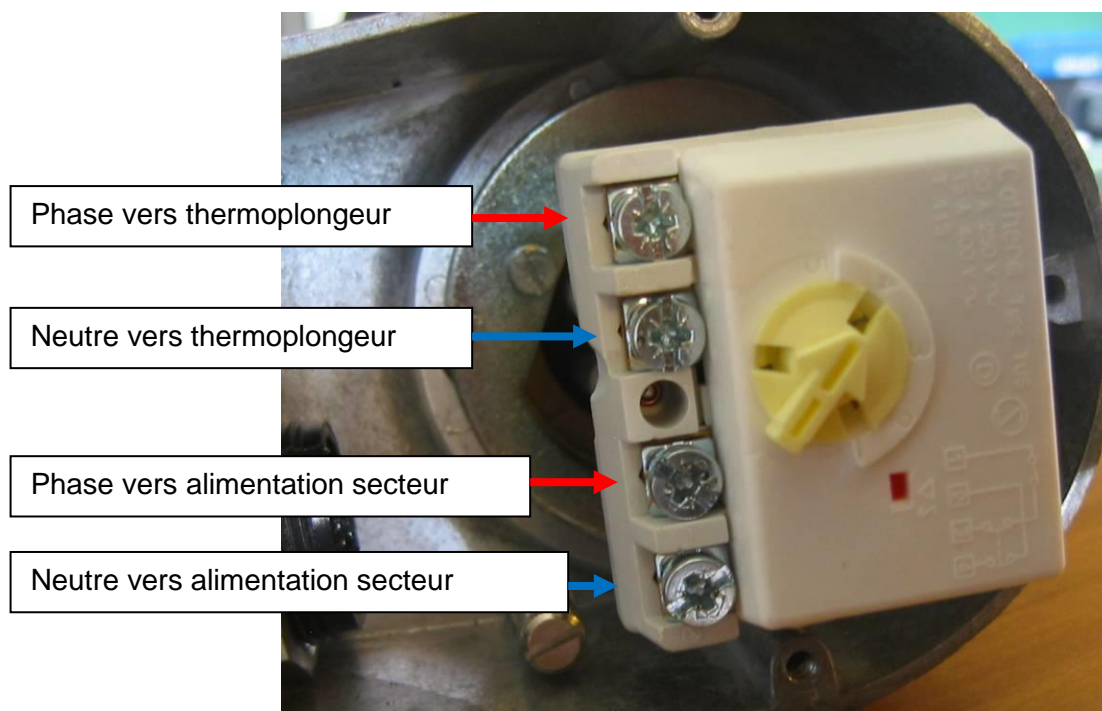
Thermostat
